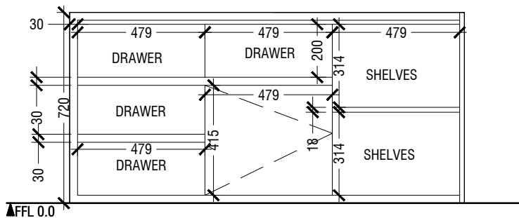
LOWER STORAGE CABINET DETAILING
