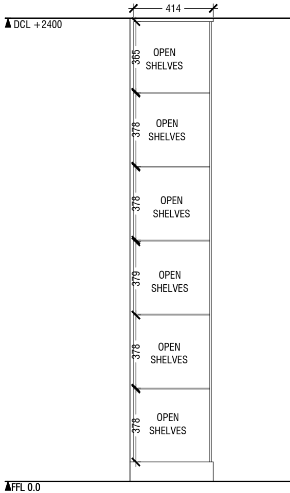
CROSS SECTION
