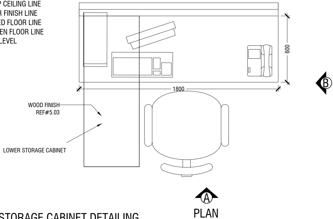
LOWER STORAGE CABINET DETAILING
